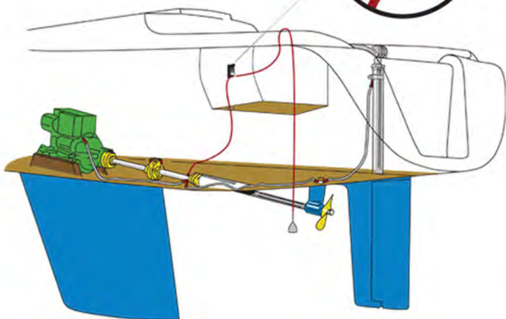
Anode Cable Mount to take the Weight
